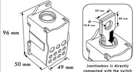
Installation Hole:85×29mm
