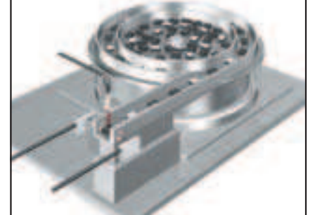
Detection of bends in electronic component leads
